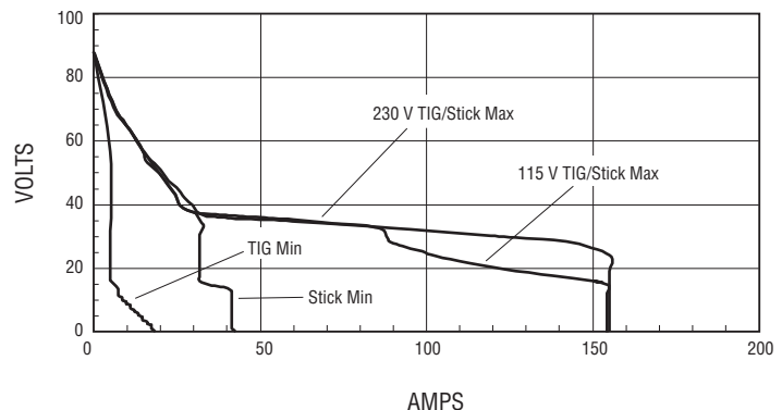
VOLT/AMP CURVES
