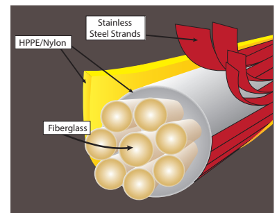
ANSI A6 cut protection from high-strength yarn
